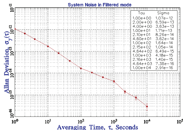
Figure 2: Noise Measurement Performance at 10 MHz
