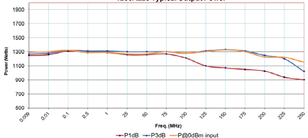
1200A225 Typical Output Power
