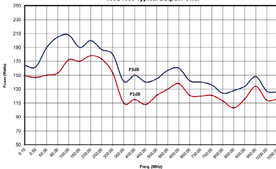
100U1000 Typical Output Power
