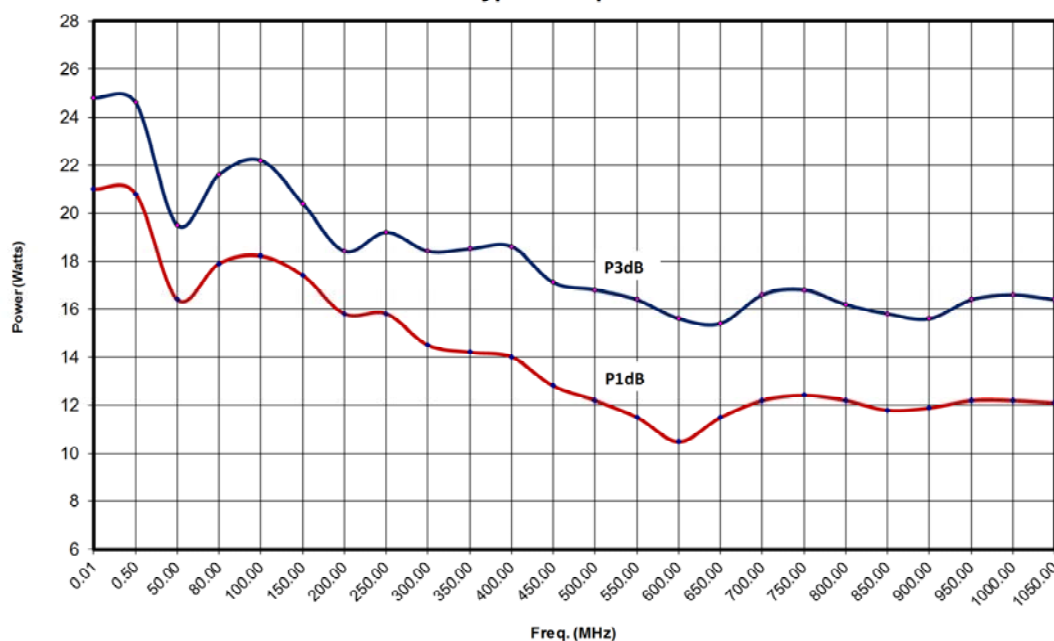
10U1000 Typical Output Power
